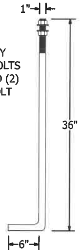
ANCHOR BOLT DETAIL
